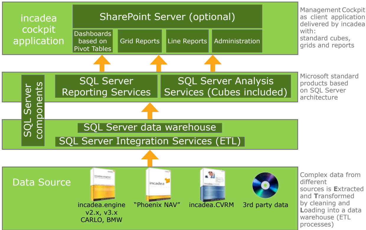
incadea.BI components and data flow
